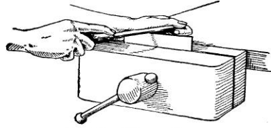
Fig. 90—Filing a Scraper
