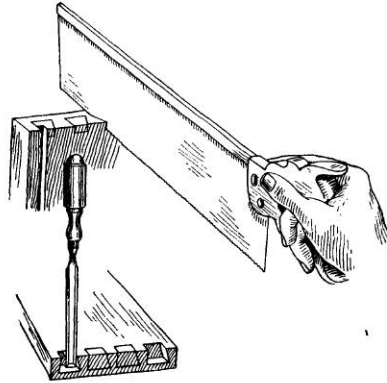
Fig. 120—Sawing the Mortises
