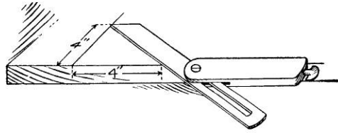
Fig. 58 —Setting Angle of T-Bevel
