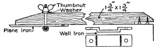
Fig- 55 — Detail of Grinding Attachment
