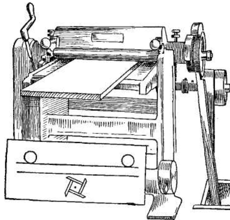
Fig. 28 —Surfacing a Board
