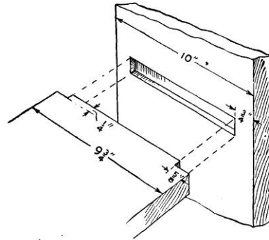
Fig. 95—Shelf Joints
