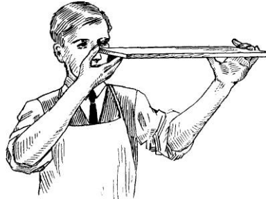
Fig. 44 —Testing for Twist
