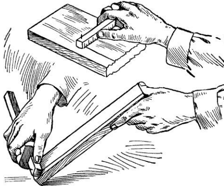
Fig. 37—Gauging for Width
