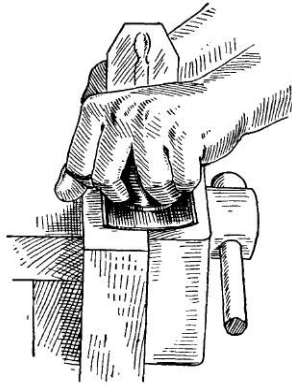
Fig. 35- Taking Shaving at High Arris
