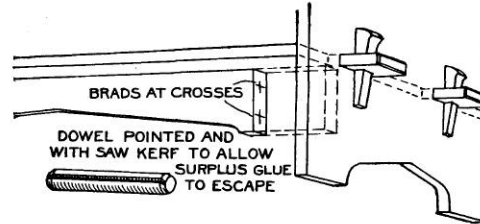
Fig. 100 —Marking Holes for Dowels
