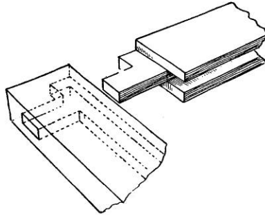
Fig. 115 —Shouldered Tenon Joint
