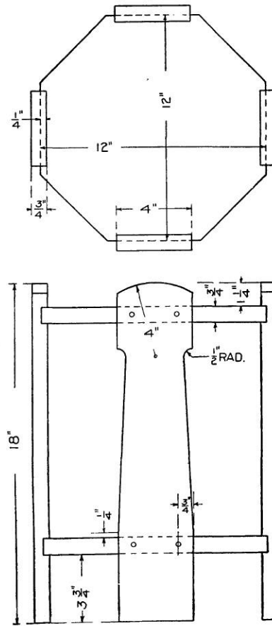
Fig. 69—Details of Taboret
