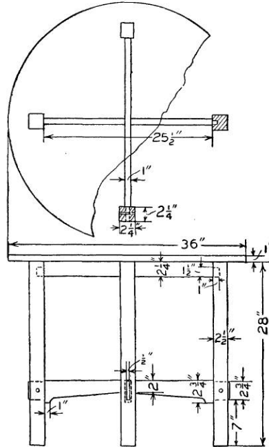
Fig. 102—Table Details
