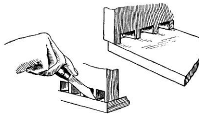
Fig. 121—Marking the Tails
