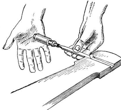
Fig. 72A—Removing Waste Material
