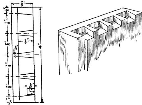
Fig. 119—Front Board Mortise
