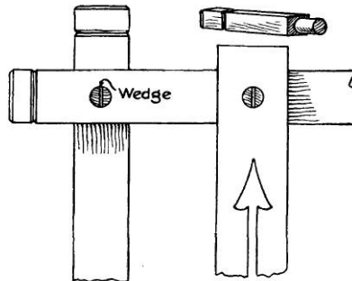
Fig. 87—Wedging the Pegs
