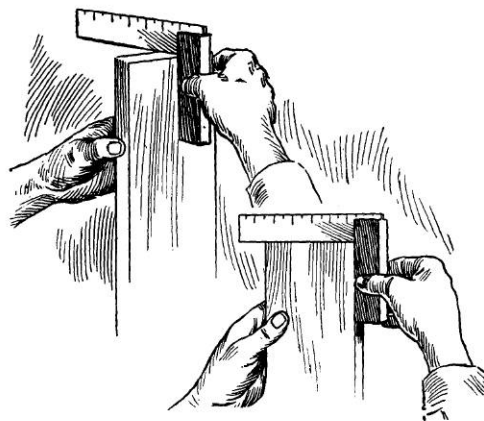
Fig. 39—End Testing
