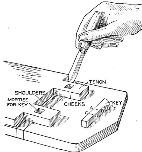
Fig. 98—Marking Mortises
