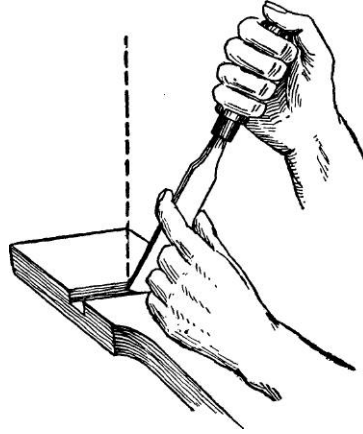
Fig. 74 —Paring the Sides
