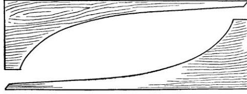
Fig. 88 —Cutting End Pieces without Waste
