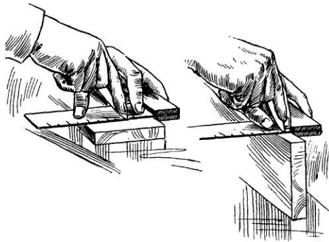
Fig. 41 — Lining Across Face and Edge
