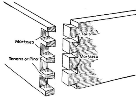
Fig 118 —Dovetail Joint
