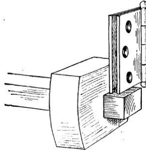
Fig. 122D —Setting Gauge for Depth
