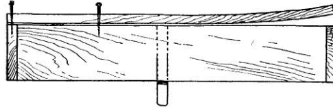
Fig. 31—Nailing Out "Dished" Board
