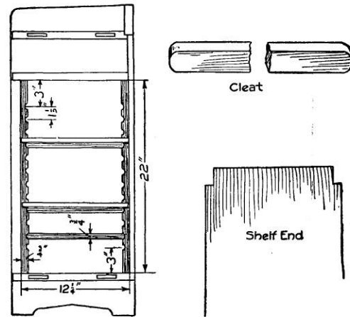
Fig. 126—Shelving Details
