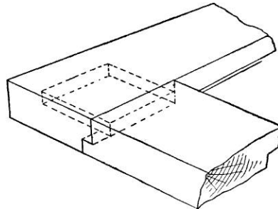
Fig. 116 — Shouldered Tenon Joint for Glass Panel
