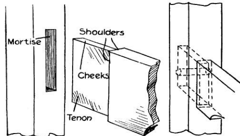
Fig. 108 —Tenon and Mortise Joint
