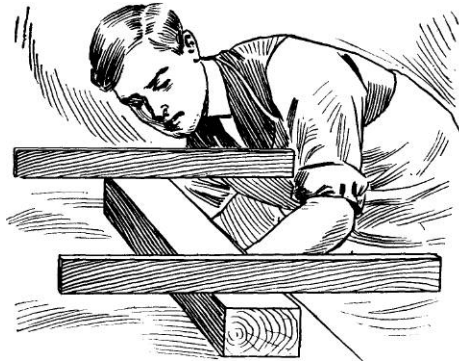
Fig. 45 —Sighting for Winding of Surface
