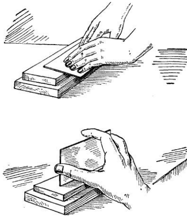
Fig. 91 — Whetting and Removing the Wire Edge
