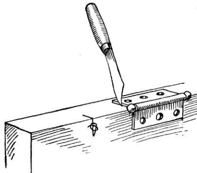
Fig. 122A — Marking Gains
