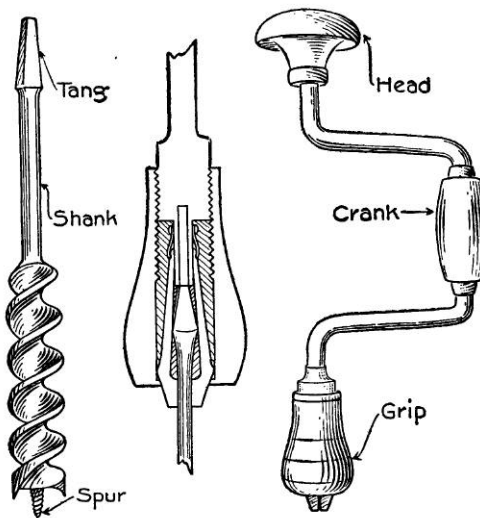
Fig. 61 — Brace and Bit
