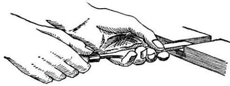
Fig. 72B—Finishing with a Paring Cut
