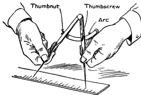
Fig. 60 — Setting Dividers
