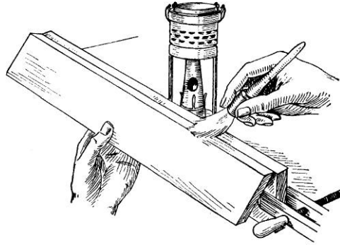
Fig. 106 — Applying Glue to the Edges
