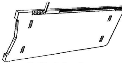
Fig. 113—Cutting a Rabbet
